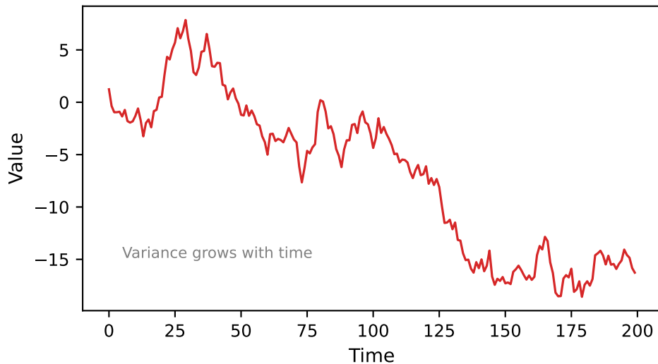
Non-Stationary: Random Walk
