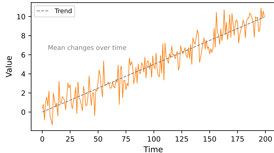
Non-Stationary: Deterministic Trend
