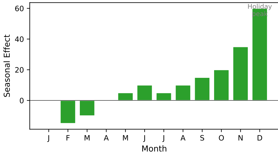
Seasonal Indices
