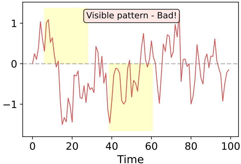
Residuals Over Time
