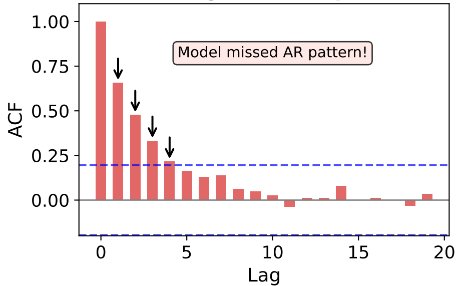
ACF: Significant Spikes!
