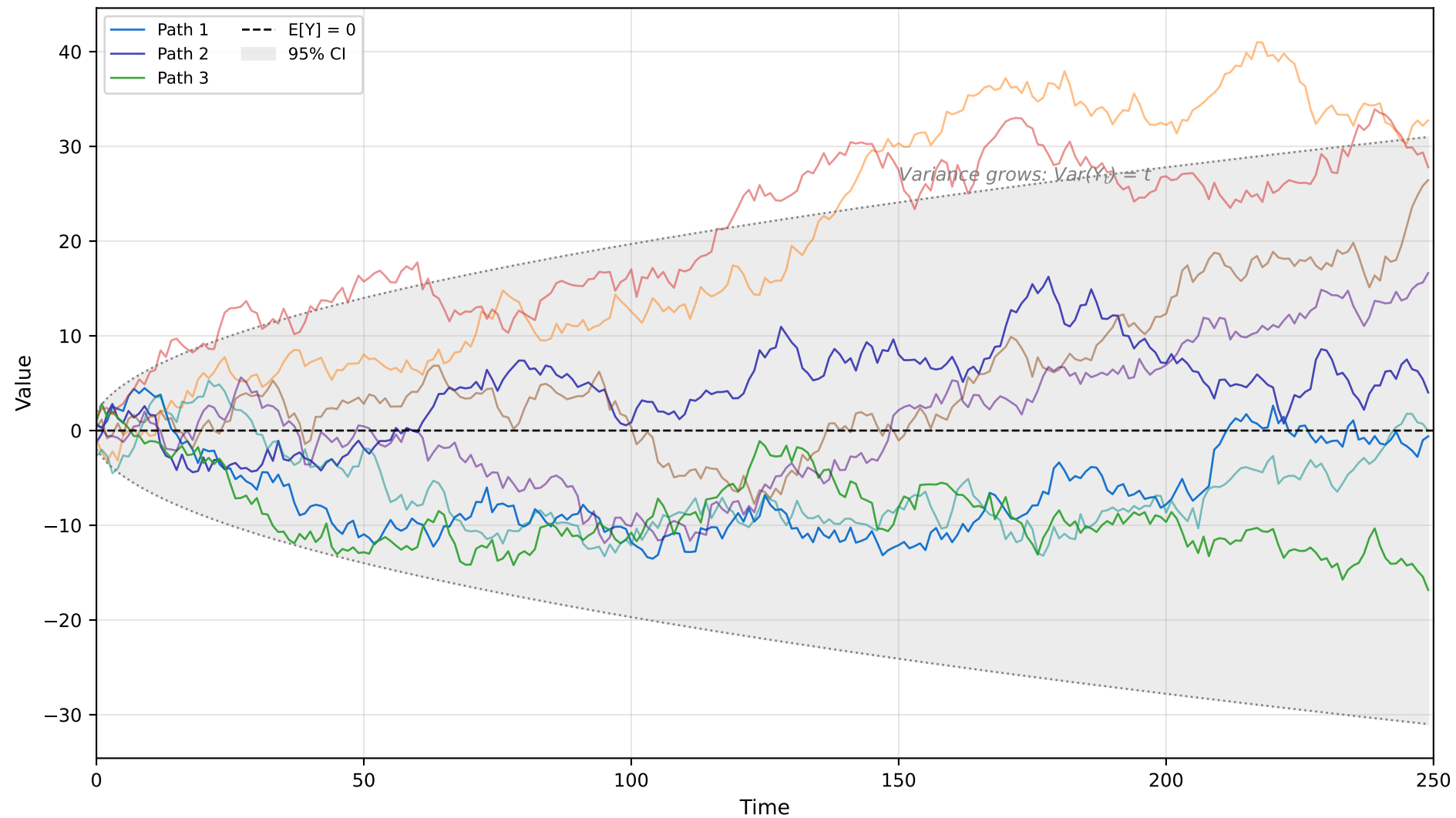
Random Walk: Y_t = Y_{t-1} + \varepsilon_t , where \varepsilon_t \sim N(0, 1)
