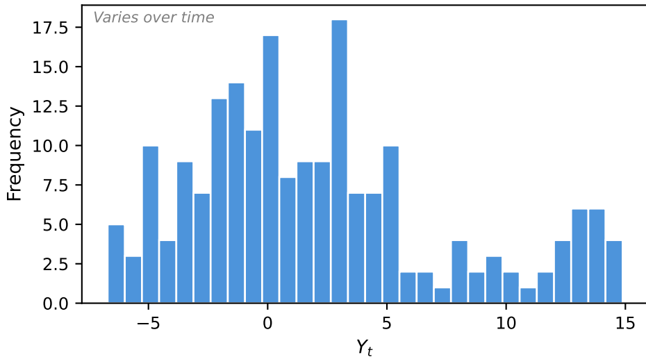
Distribution of Original
