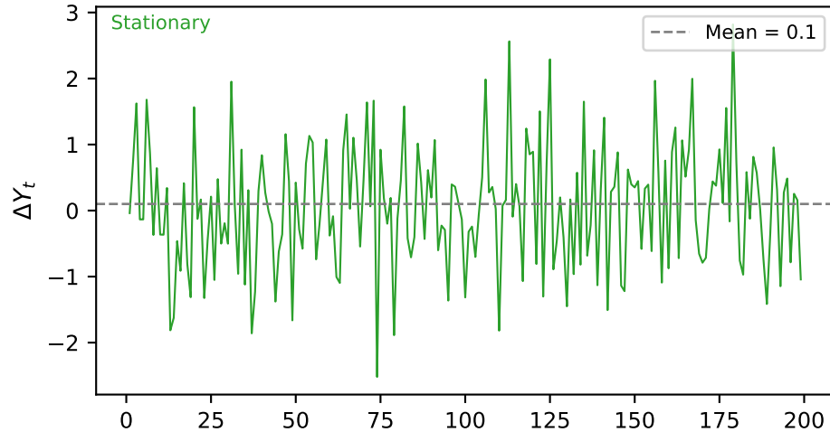
Distribution of First Difference
