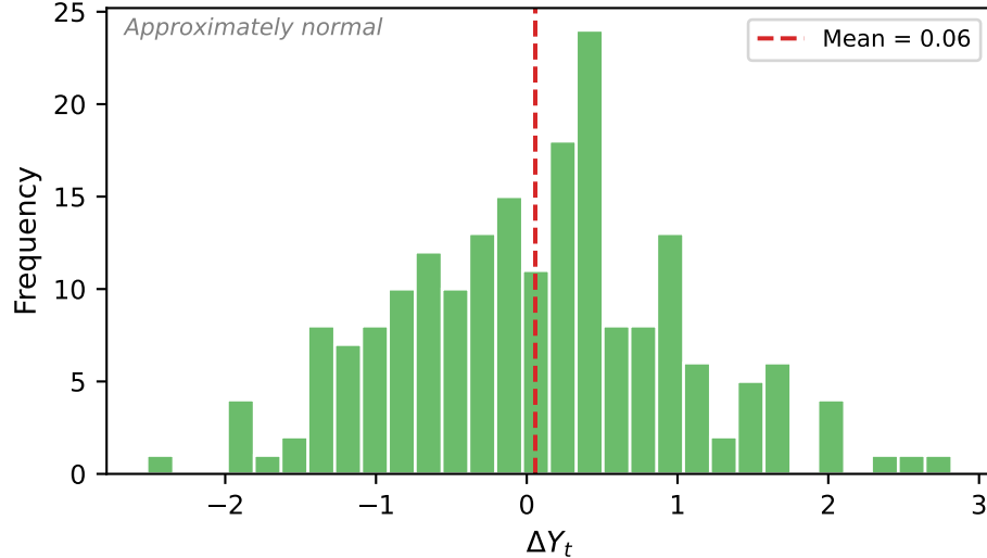
Distribution of First Difference
