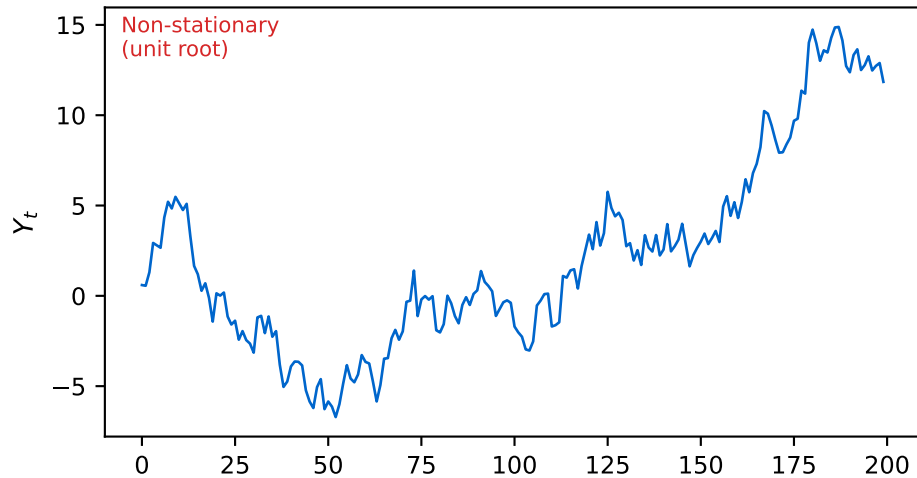
Distribution of Original
