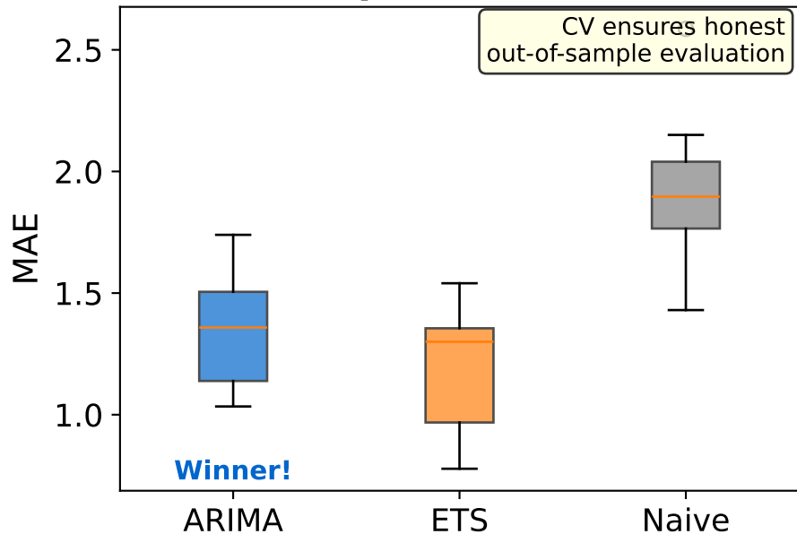
Model Comparison (10-Fold CV)
