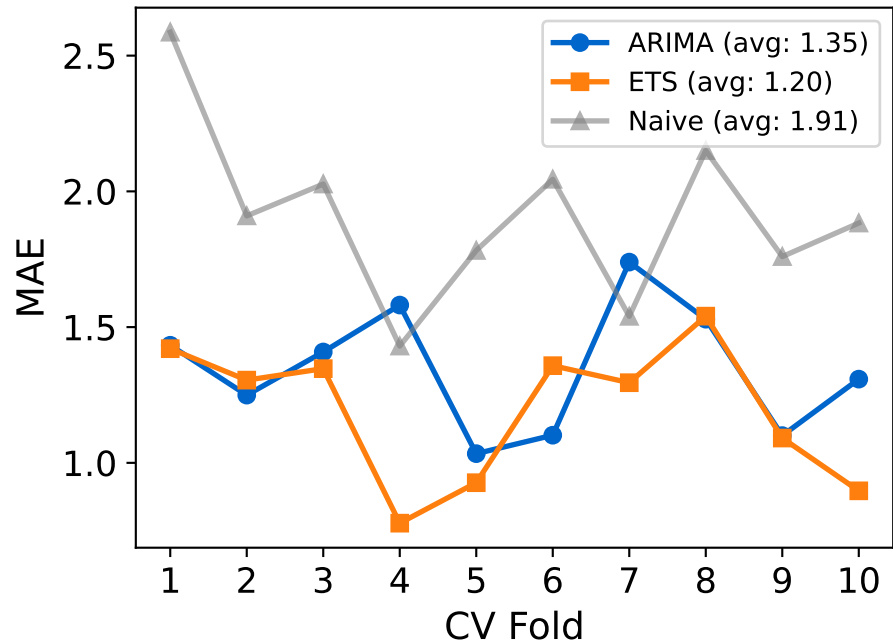
Error Across CV Folds
