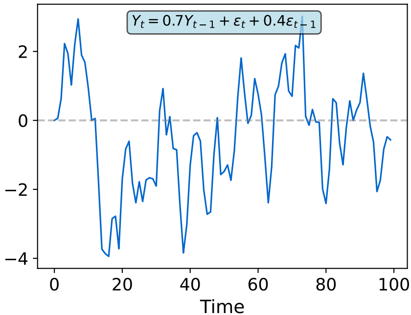
ARMA(1,1) Simulated Series
