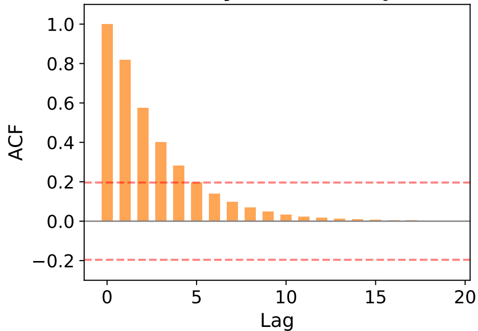
ACF (Decays - Not Sharp Cut)
