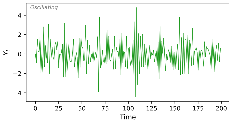
AR(1): \phi = -0.7
