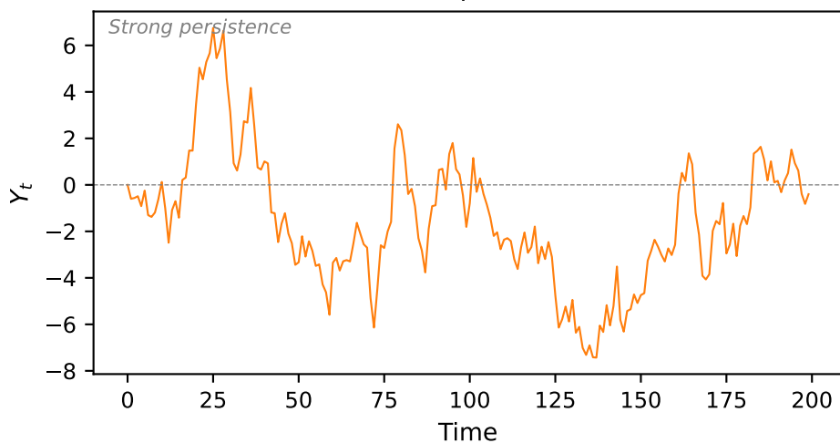
AR(1): \phi = 0.95
