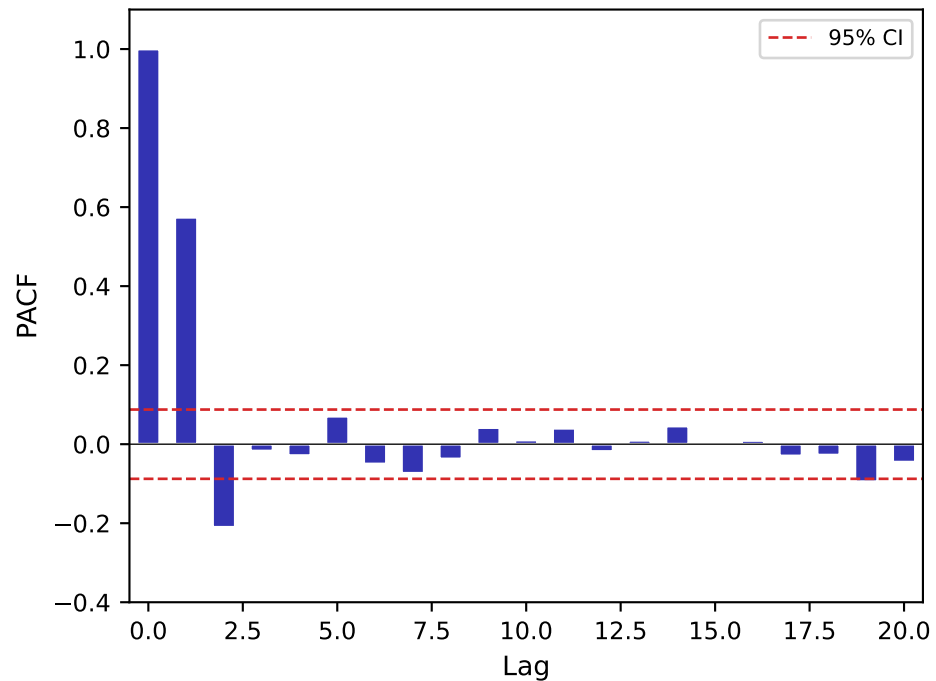
Partial Autocorrelation Function (PACF)
