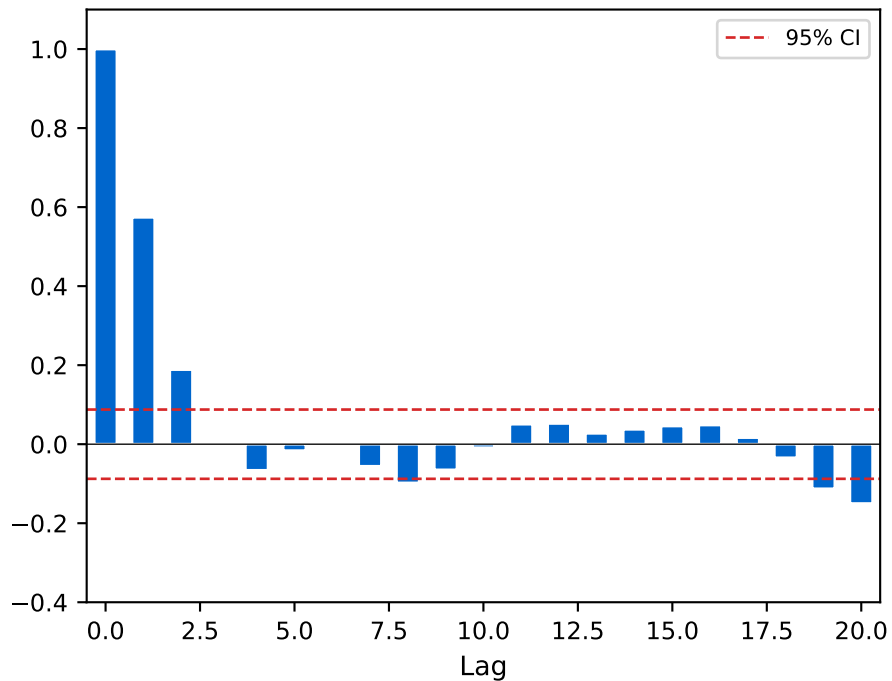
Autocorrelation Function (ACF)
