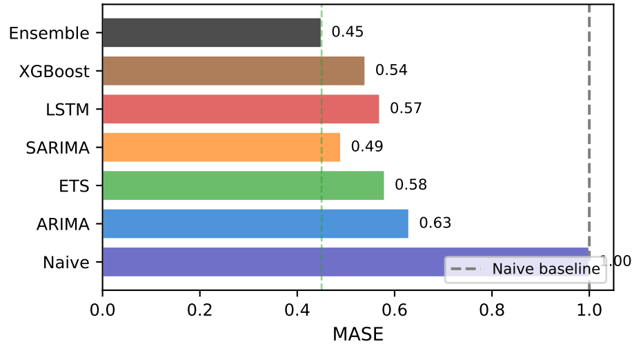
Mean Absolute Scaled Error
