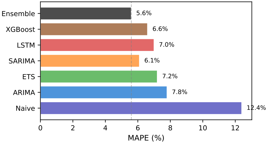
Mean Absolute Percentage Error
