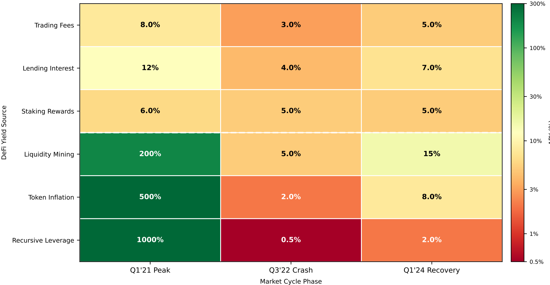
Yield Source Survival Heatmap: Average APY by Market Cycle
