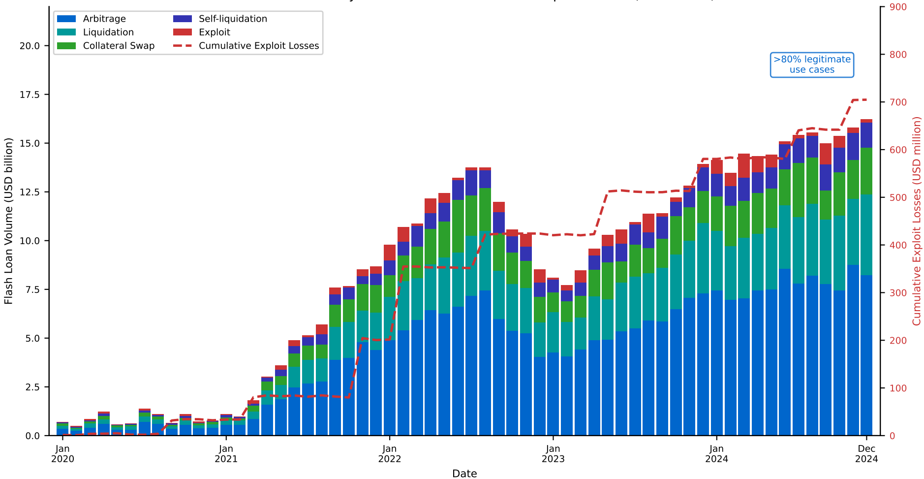
Flash Loan Volume by Use Case with Cumulative Exploit Losses (2020-2024)
