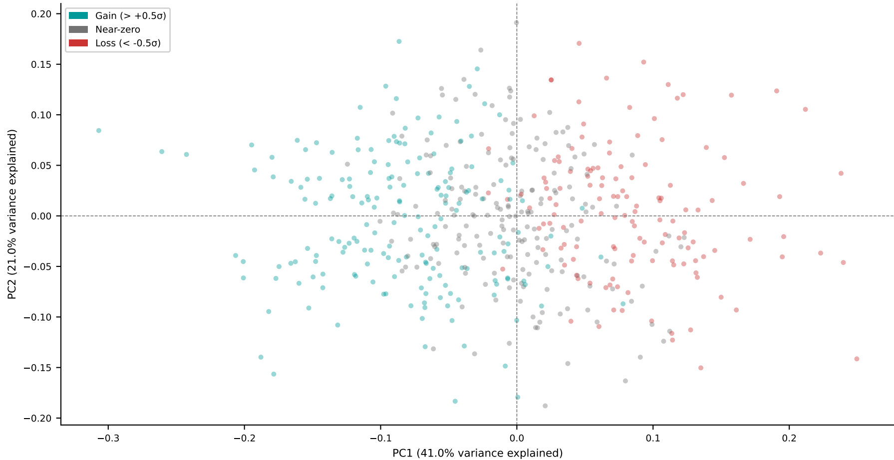
PCA Factor Biplot: Scenarios Colored by Portfolio P&L
