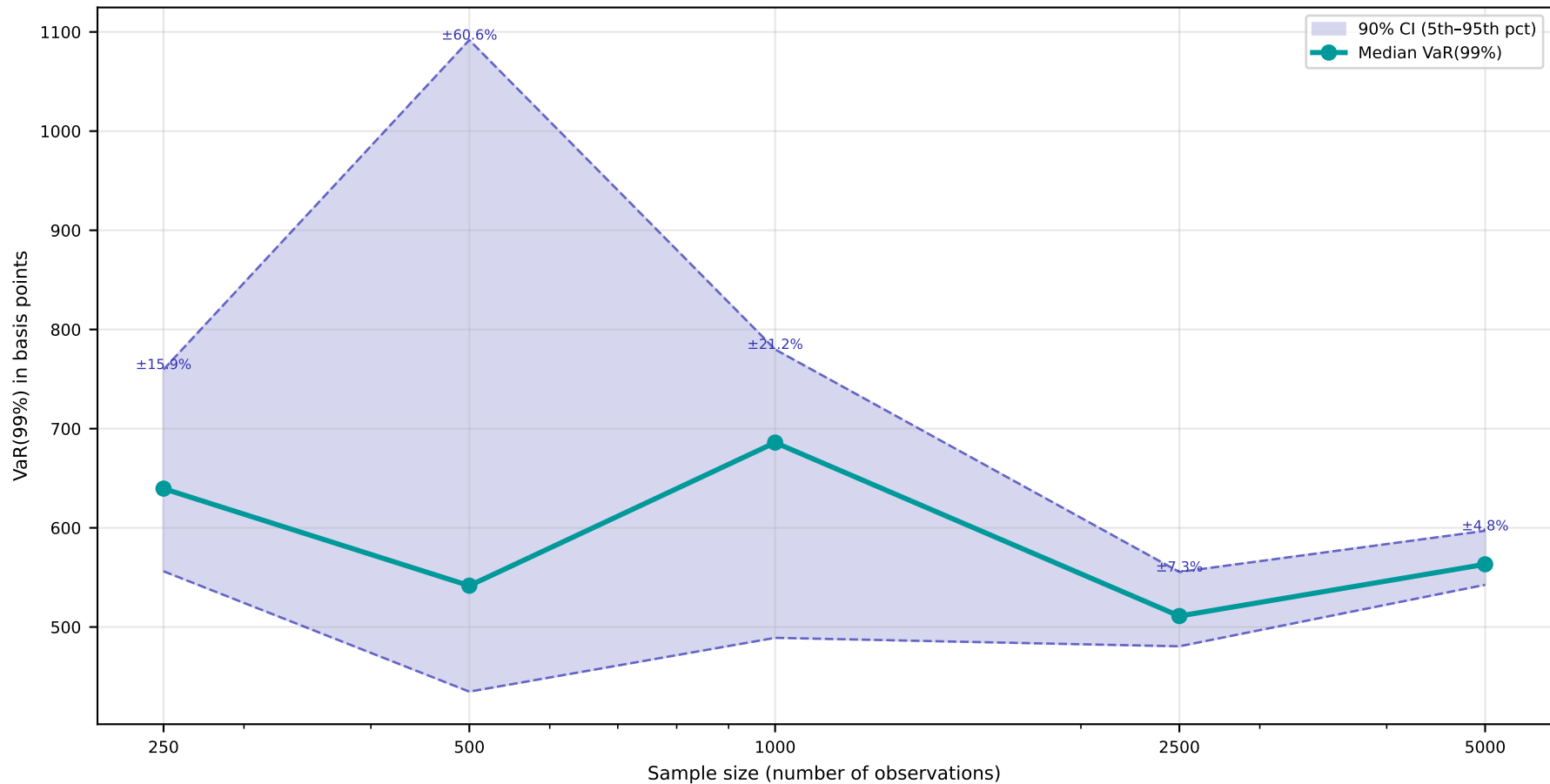
Bootstrap 90% Confidence Interval for VaR(99%)
