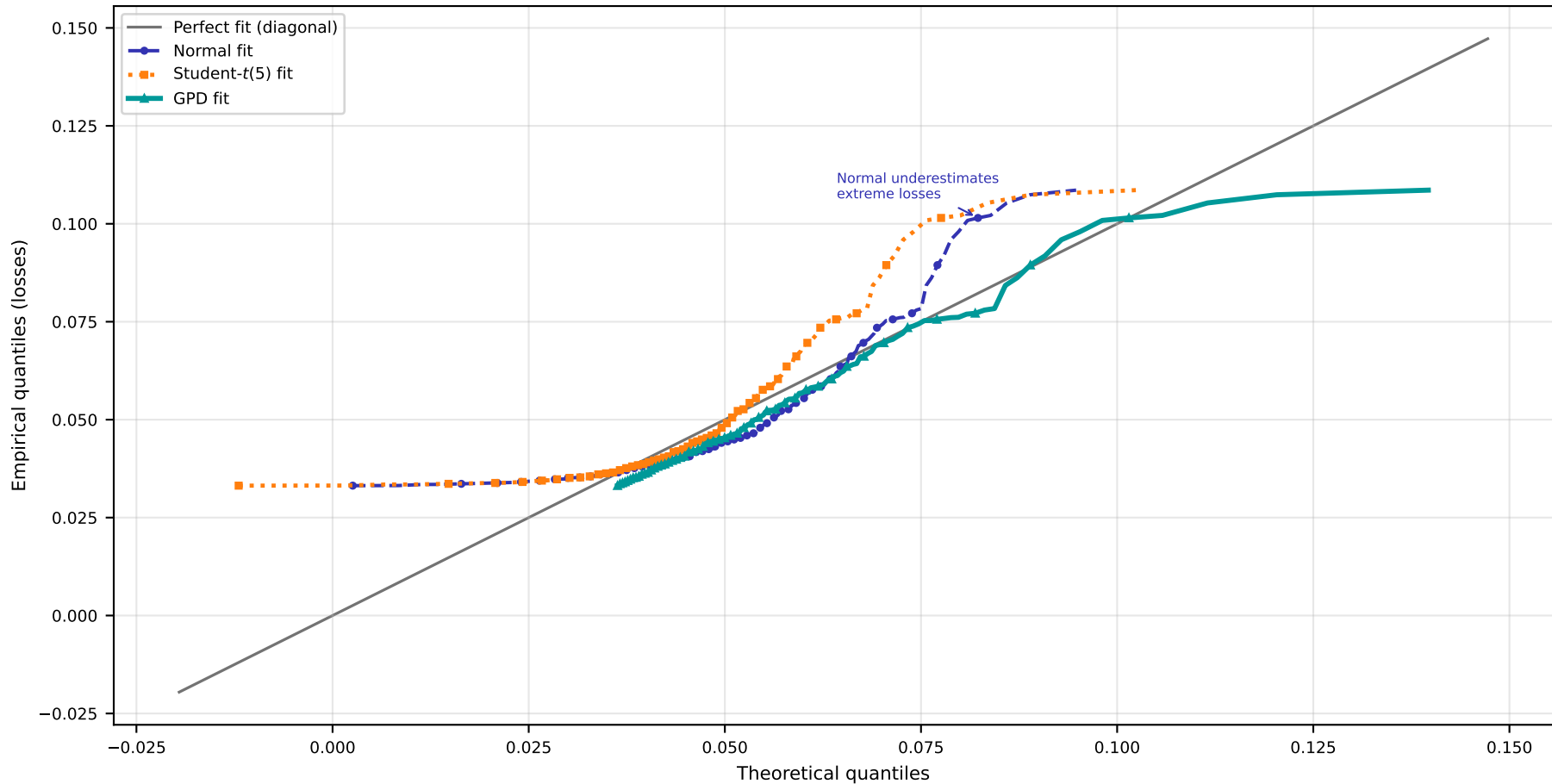
QQ Plot: Tail Model Comparison (Lower 5%)
