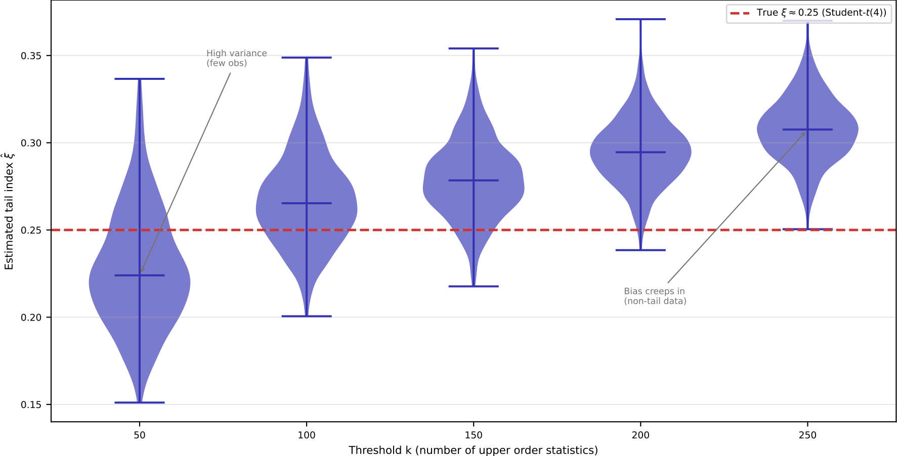
Hill Estimator Stability: Sampling Distribution Across Thresholds
