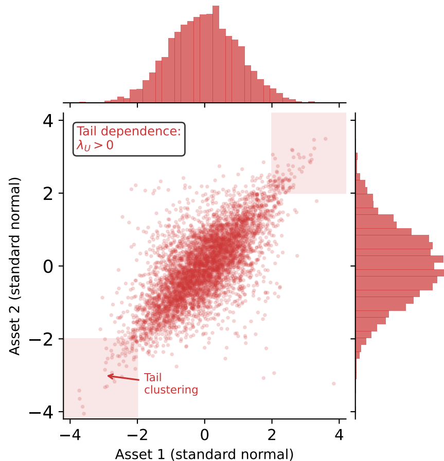
Student-t Copula ( \rho = 0.7, df = 3 )
