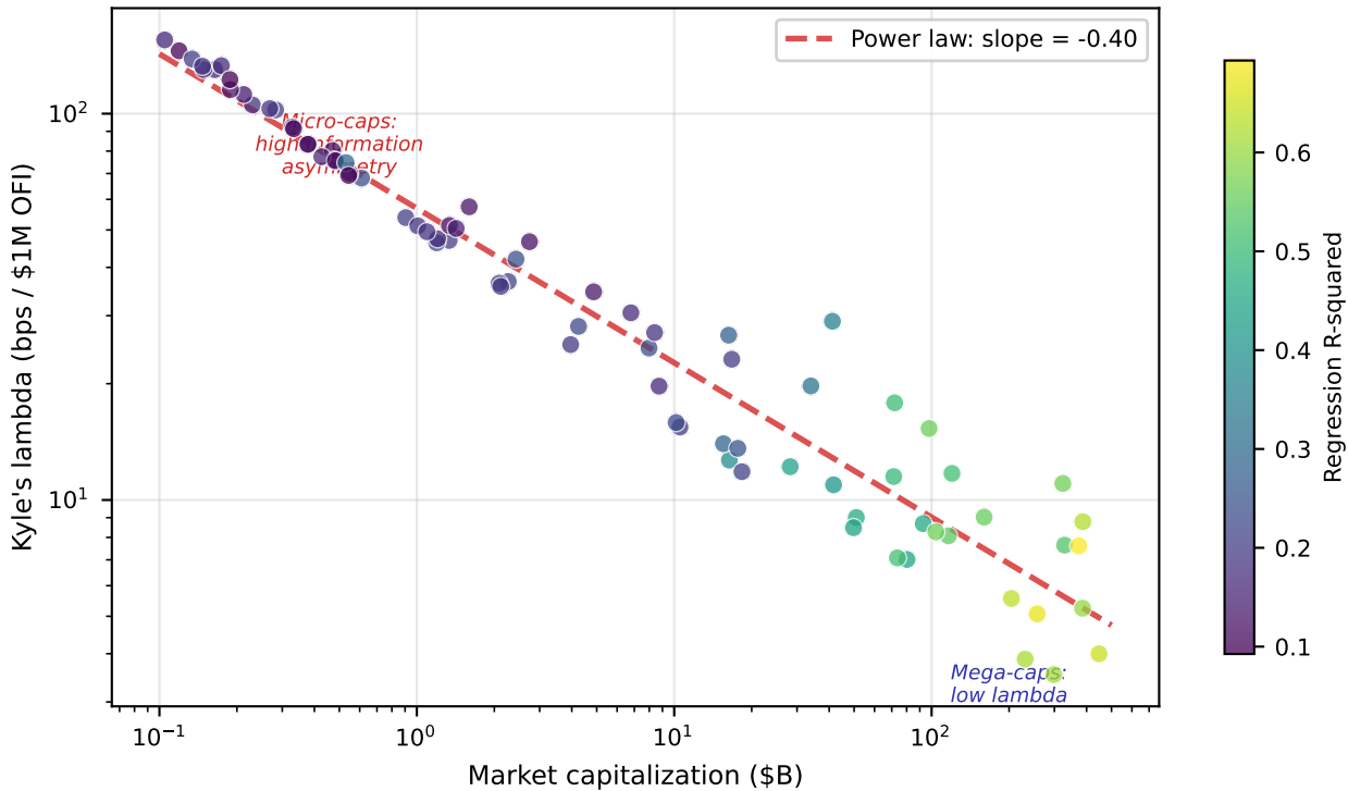
Kyle's Lambda vs Market Cap (Cross-Section)
