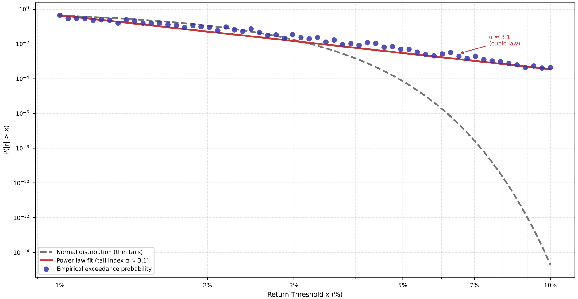
Tail Risk Exceedance Plot: Fat Tails Far Exceed Normal Distribution Predictions
