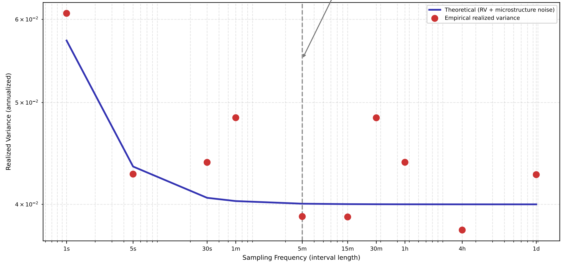
Microstructure Noise Signature Plot: RV Inflates at High-Frequency Sampling
