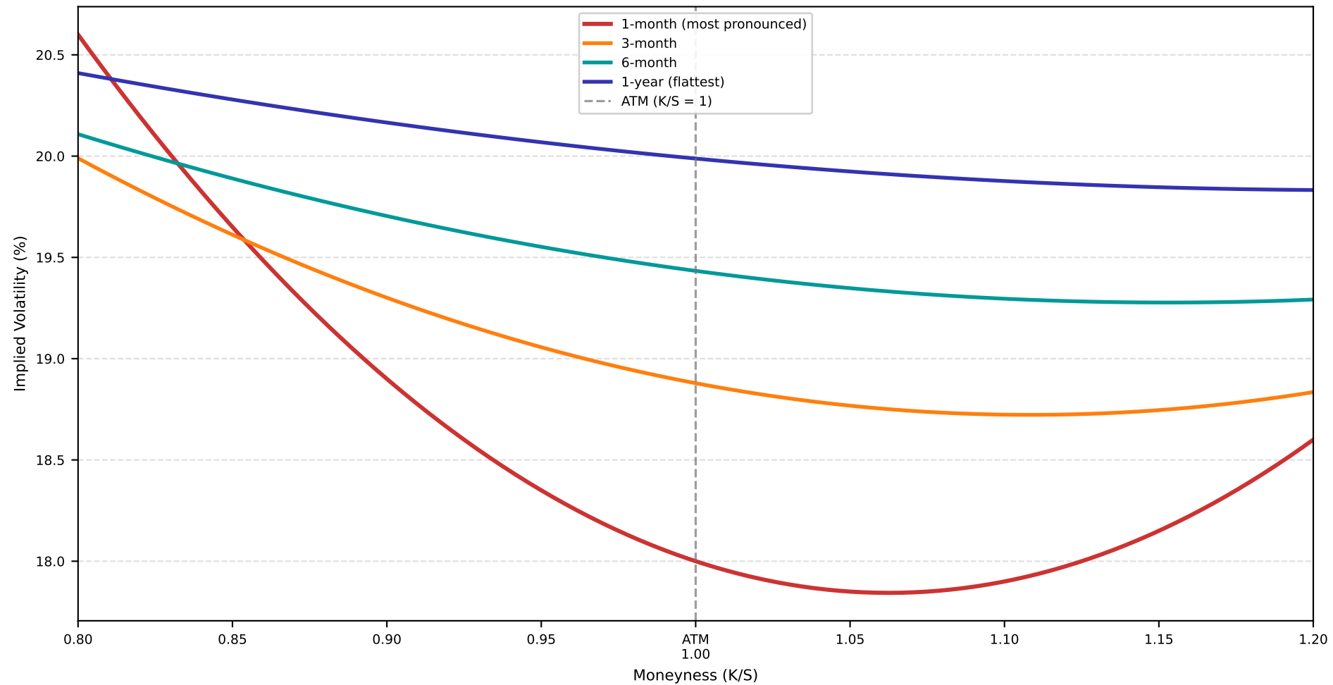
Volatility Smile by Maturity: Pronounced Smile Flattens as Expiry Lengthens
