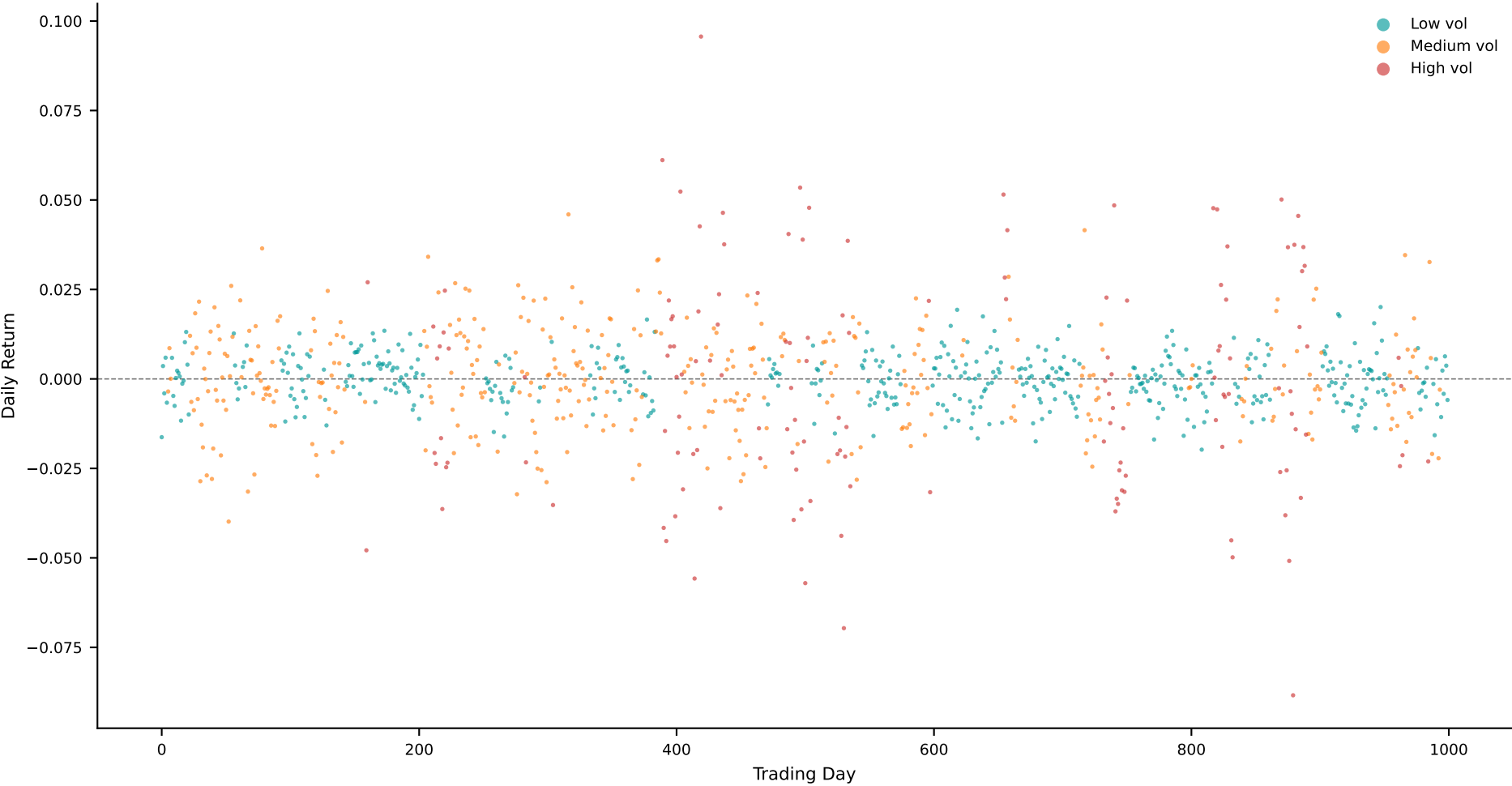
Volatility Clustering: Daily Returns by GARCH Regime
