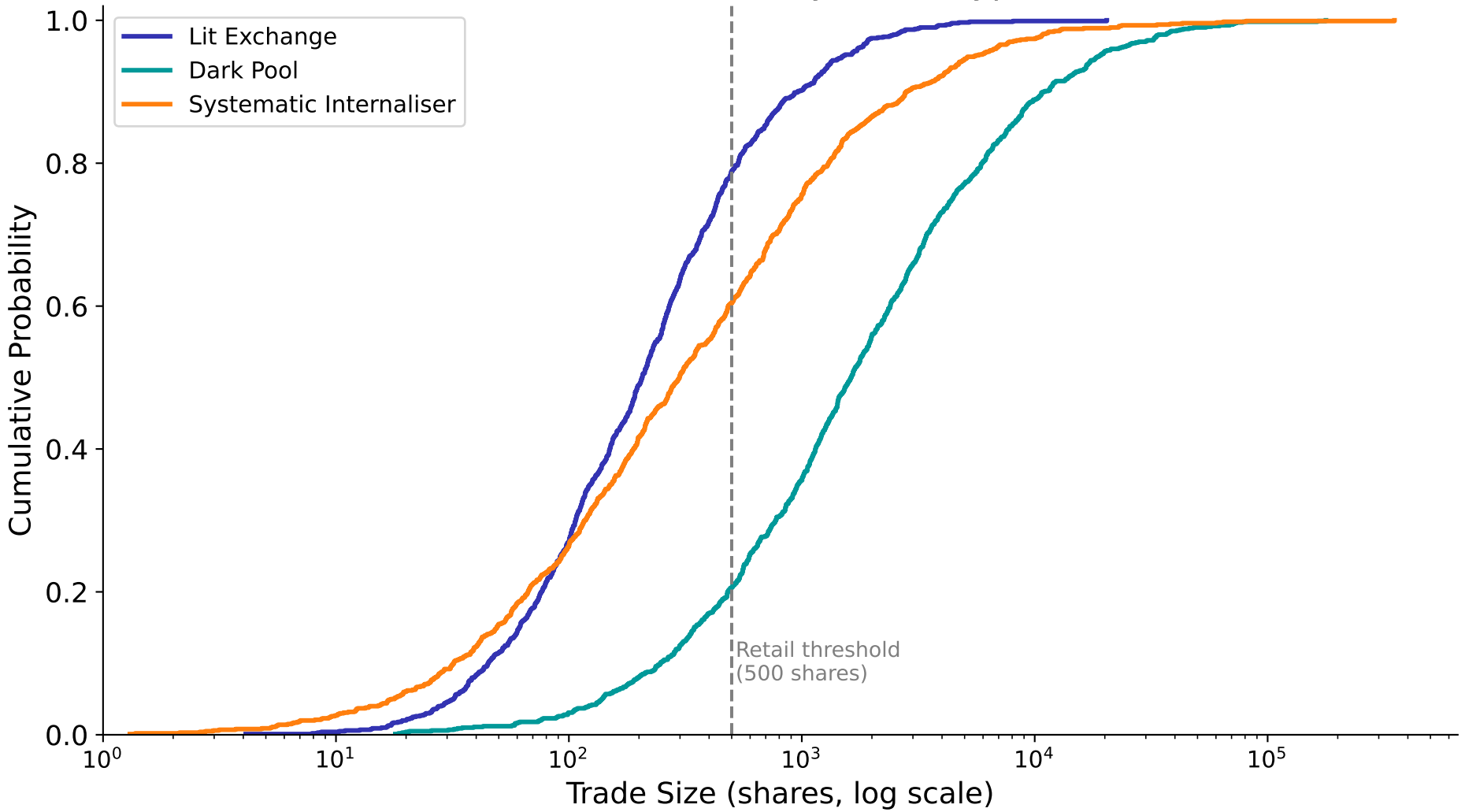
Trade Size Distribution by Venue Type (ECDF)
