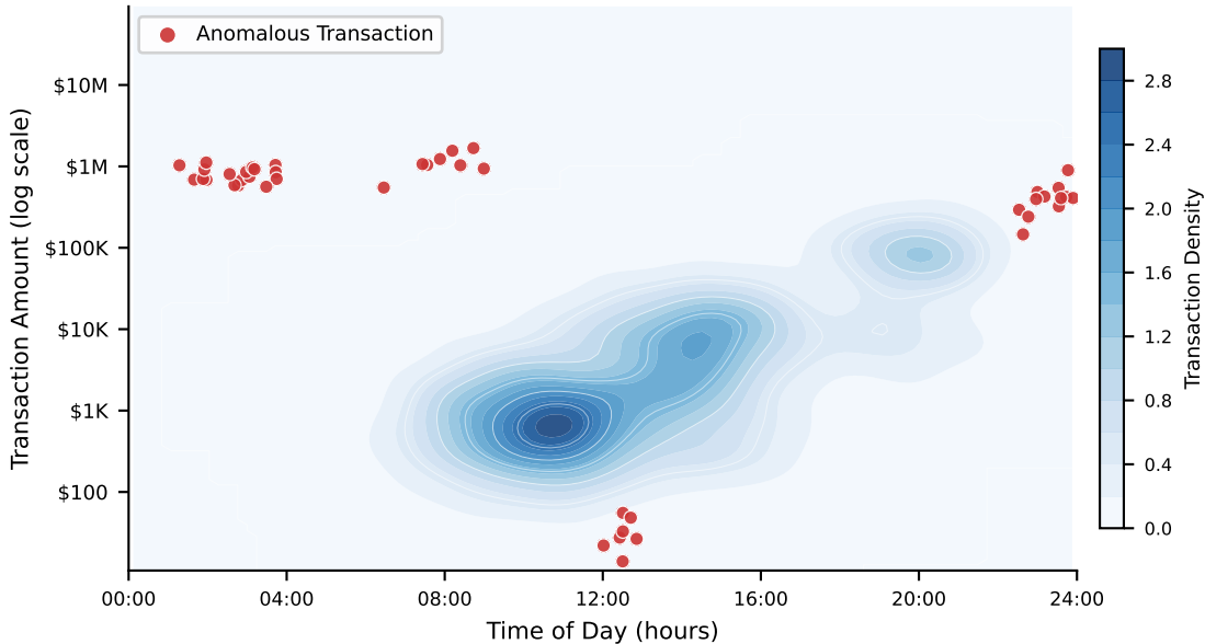
Transaction Anomaly Detection: Amount vs Time of Day (Contour = normal density; red dots = anomalies)
