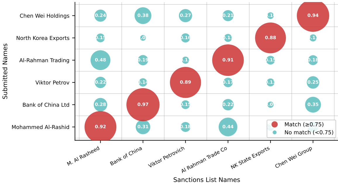
Name Screening: Jaro-Winkler Similarity Matrix (Bubble size = similarity; red = above 0.75 threshold)
