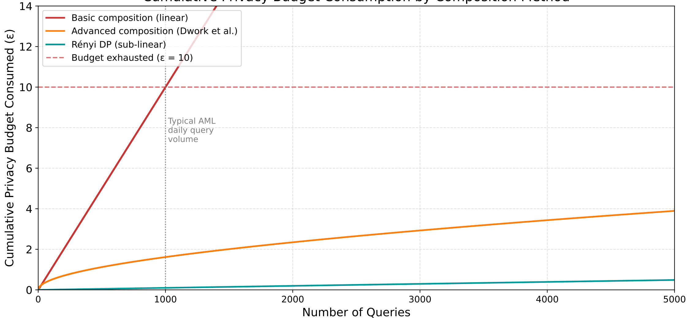
Cumulative Privacy Budget Consumption by Composition Method
