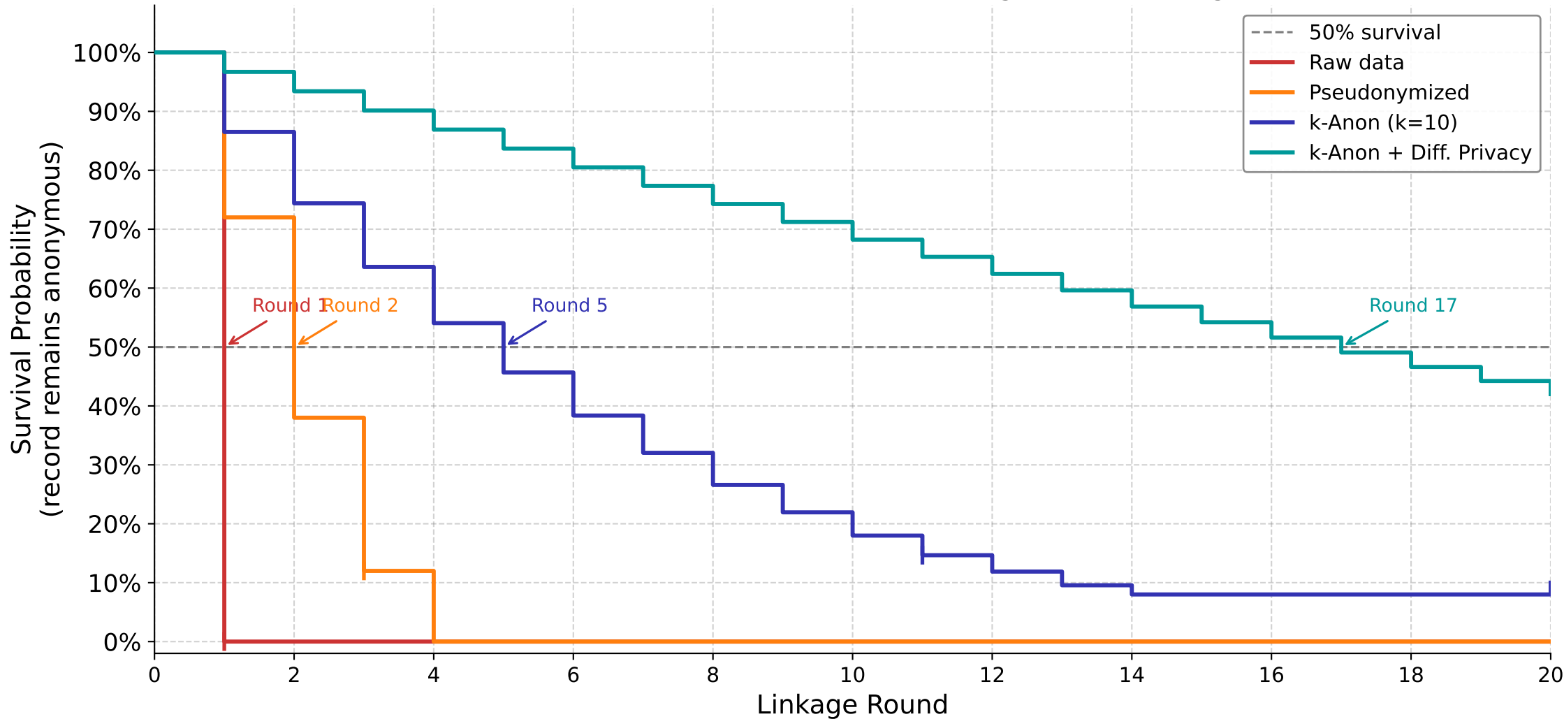
Re-Identification Survival Curves Under Progressive Linkage Attack
