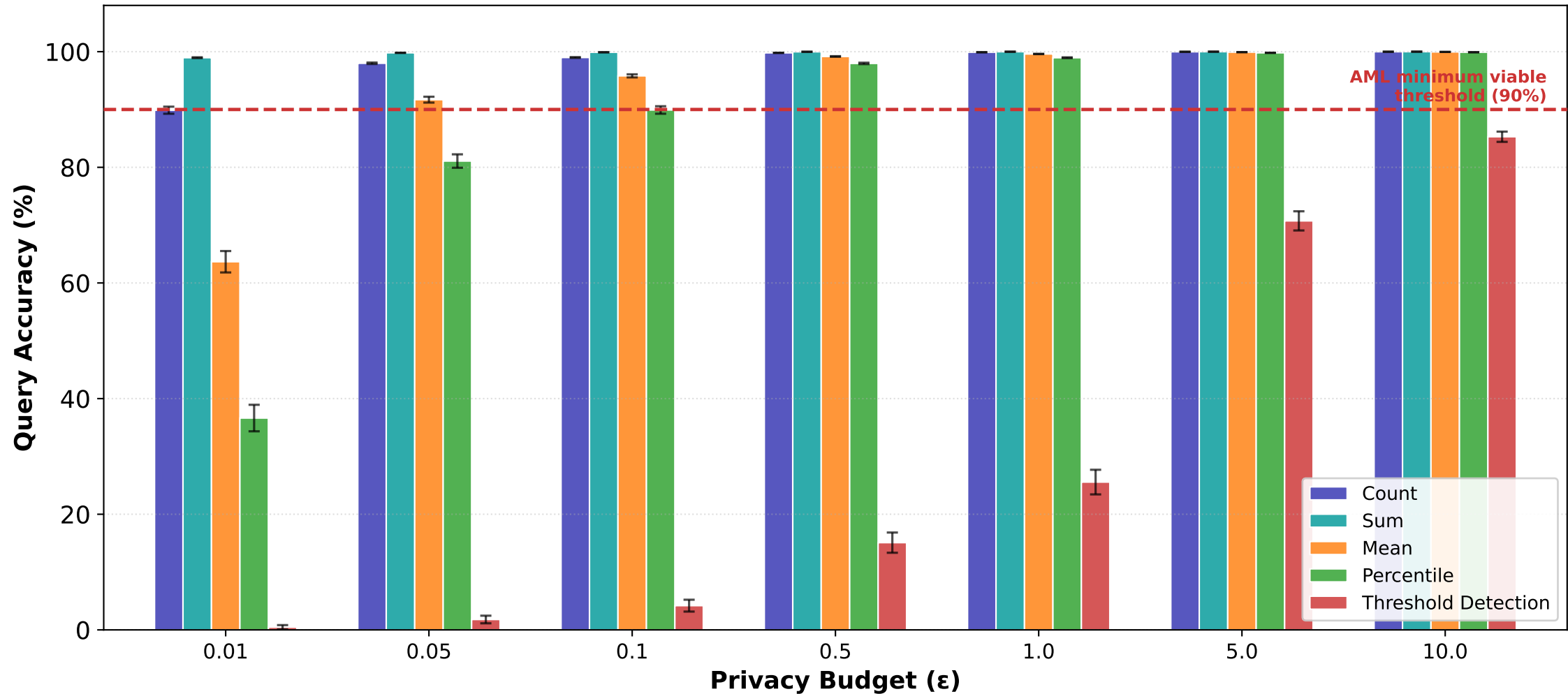
Differential Privacy: Query Accuracy vs Privacy Budget ( \epsilon ) 1,000 simulated trials per ( \epsilon , query type), 95% CI shown
