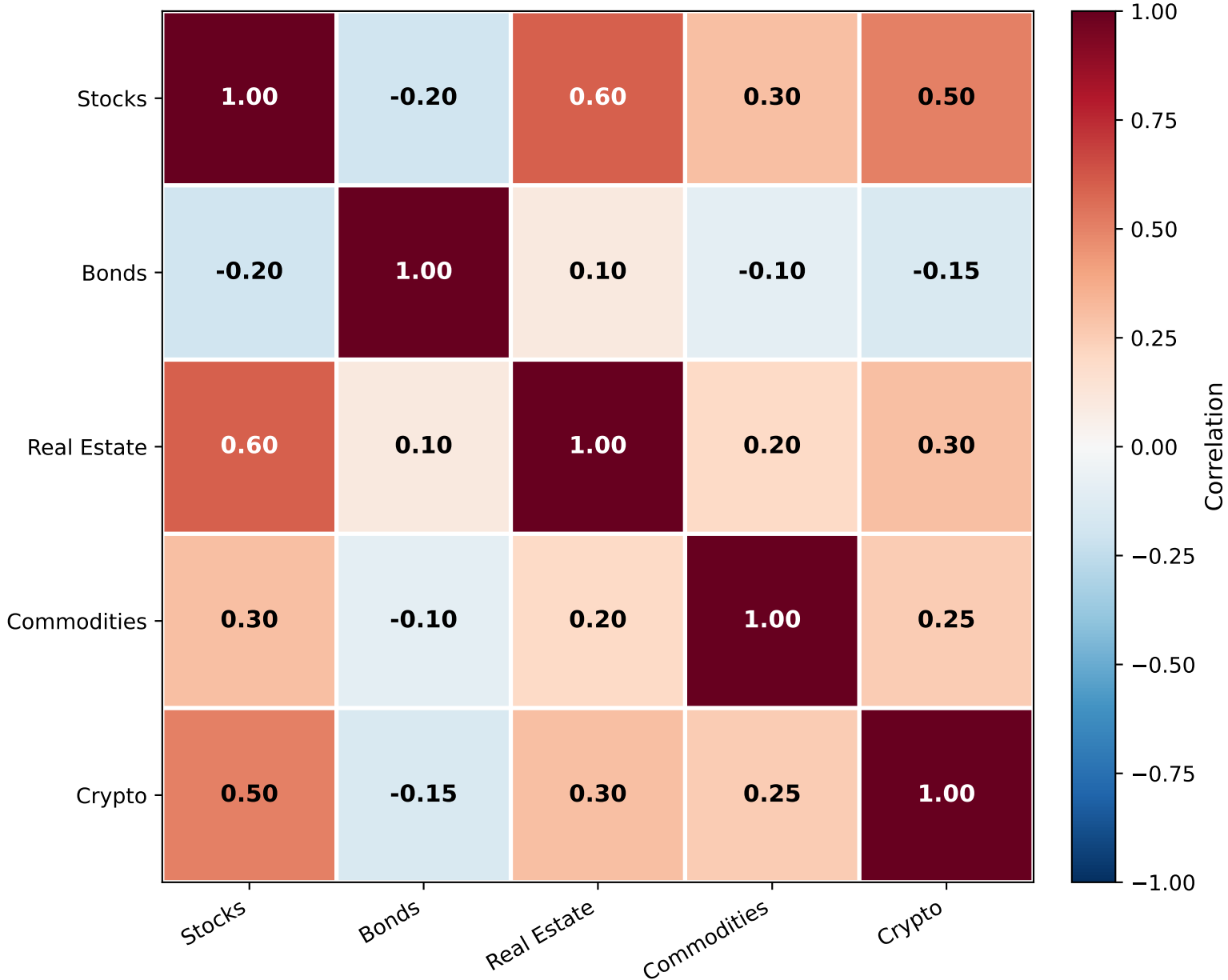
Asset Correlation Matrix (5 Asset Classes)
