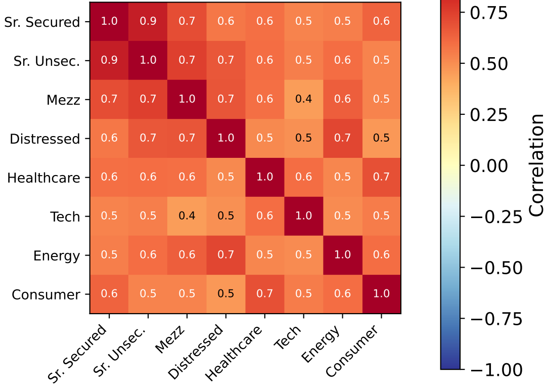
Crisis Regime Correlation Matrix
