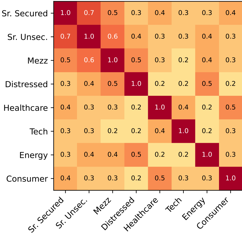
Normal Regime Correlation Matrix
