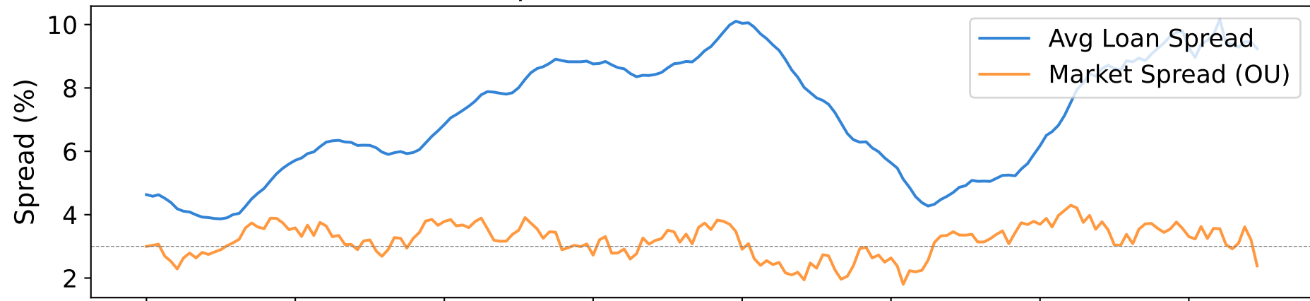
Credit Spreads: Simulated Loan Portfolio
