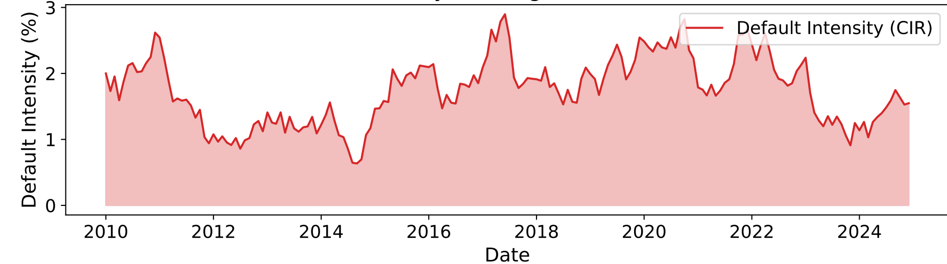
Default Intensity: Cox-Ingersoll-Ross Process
