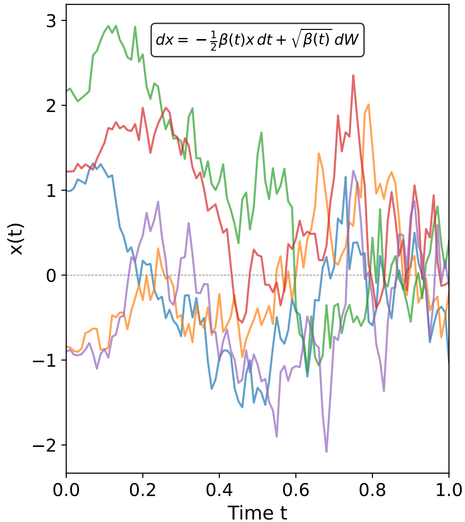
Forward SDE: Data \rightarrow Noise
