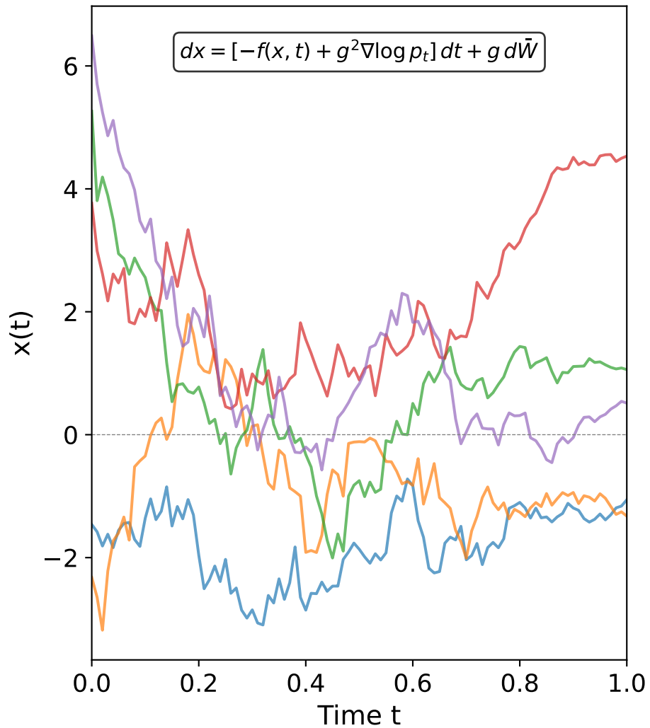
Reverse SDE: Noise \rightarrow Data
