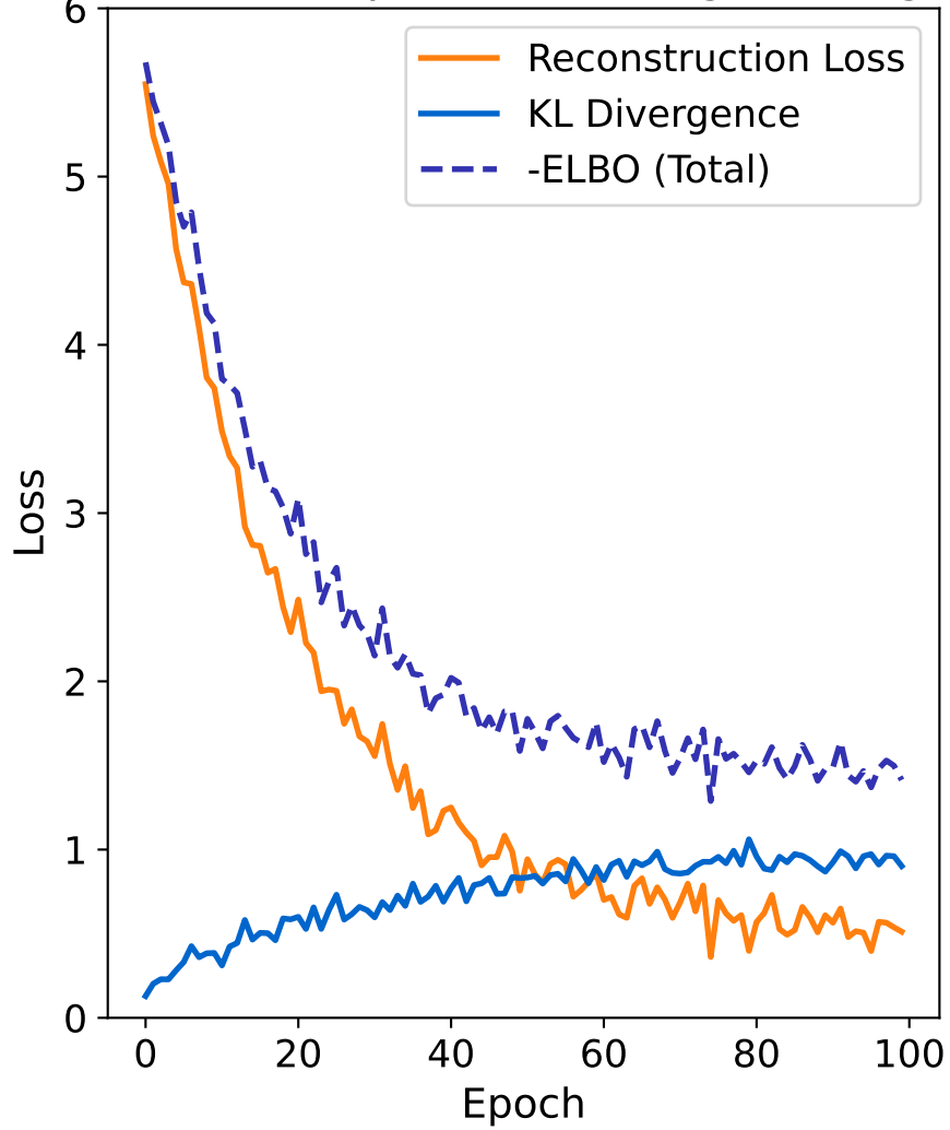
ELBO Components During Training
