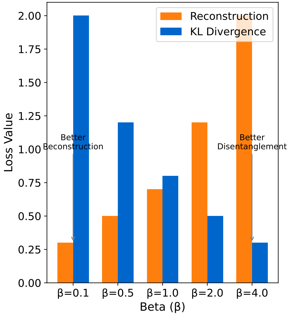
Beta-VAE Trade-off
