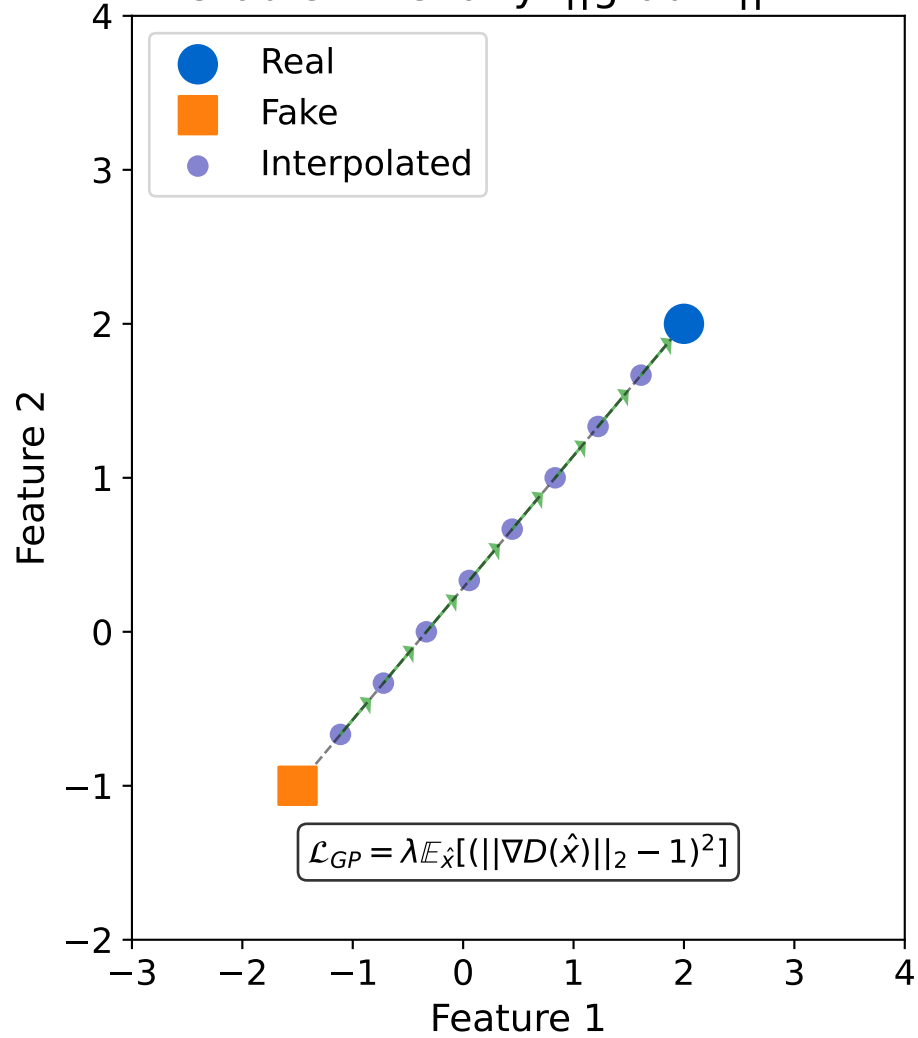
Gradient Penalty: \|\text{grad } D\| = 1
