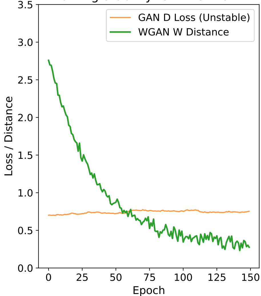
Training Stability: GAN vs WGAN
