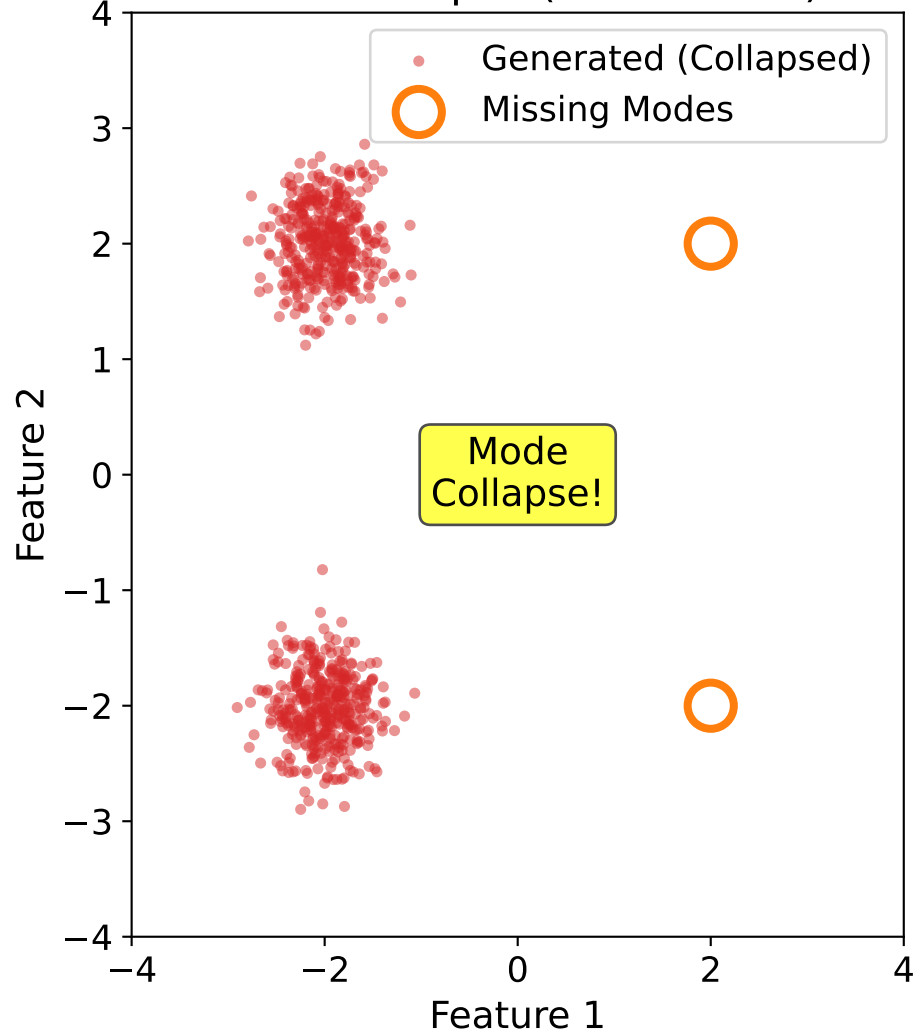
Mode Collapse (GAN Failure)
