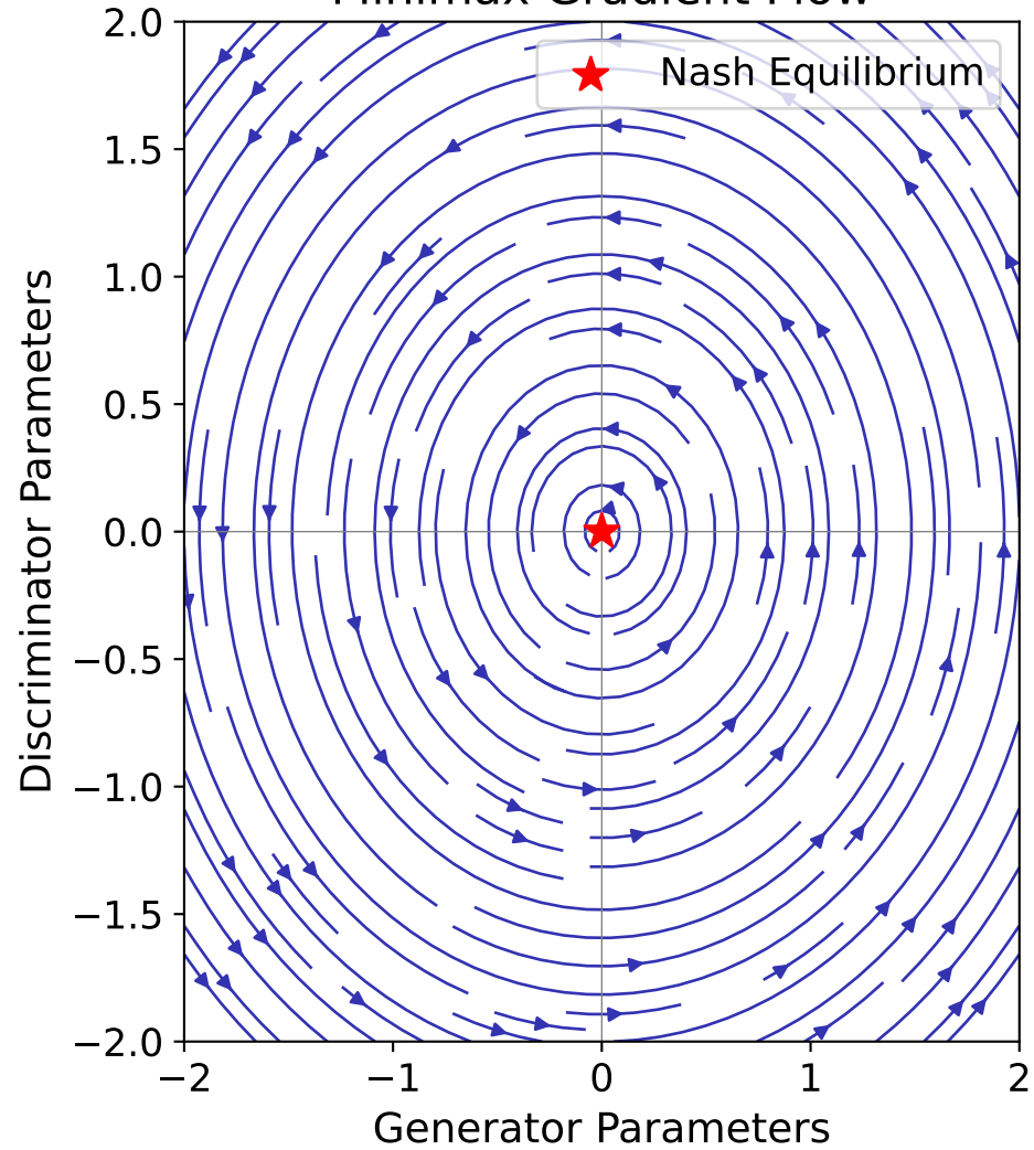
Minimax Gradient Flow
