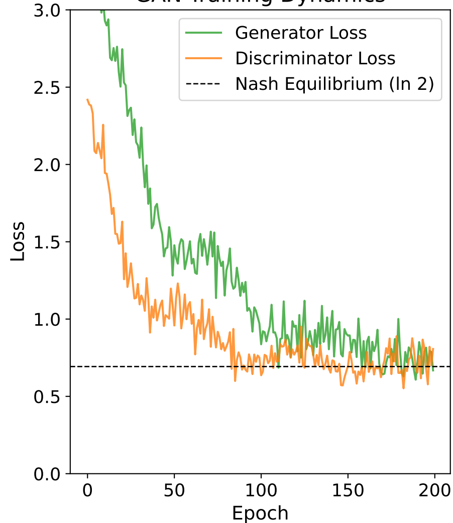
GAN Training Dynamics
