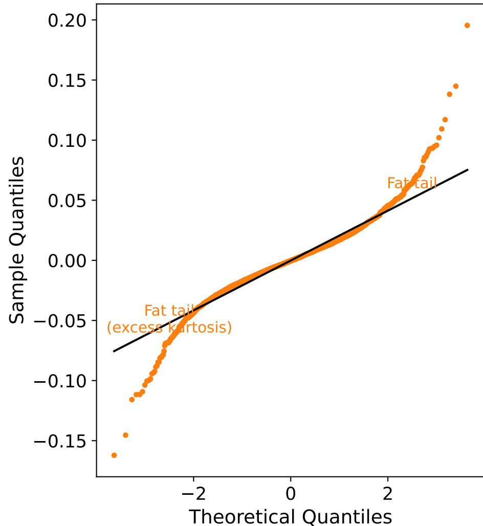
Q-Q Plot: Financial vs Normal
