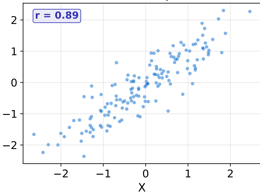
r = +0.9 (stark positiv)
