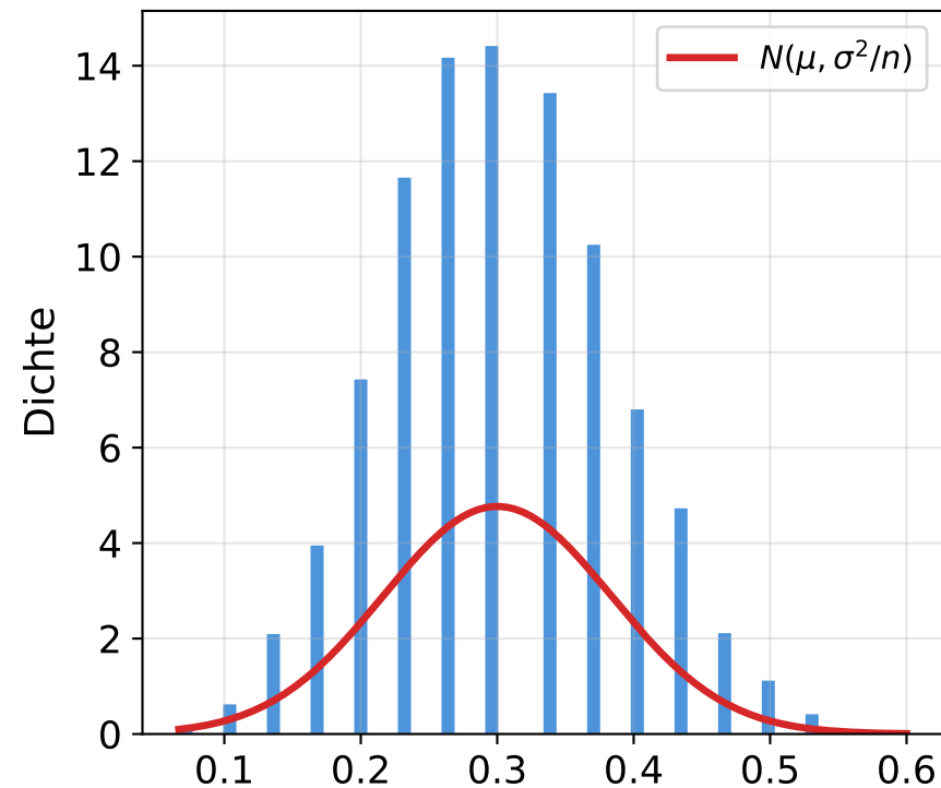
Bernoulli(0,3)
