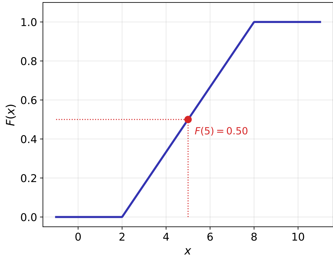
CDF: X \sim U(2, 8)
