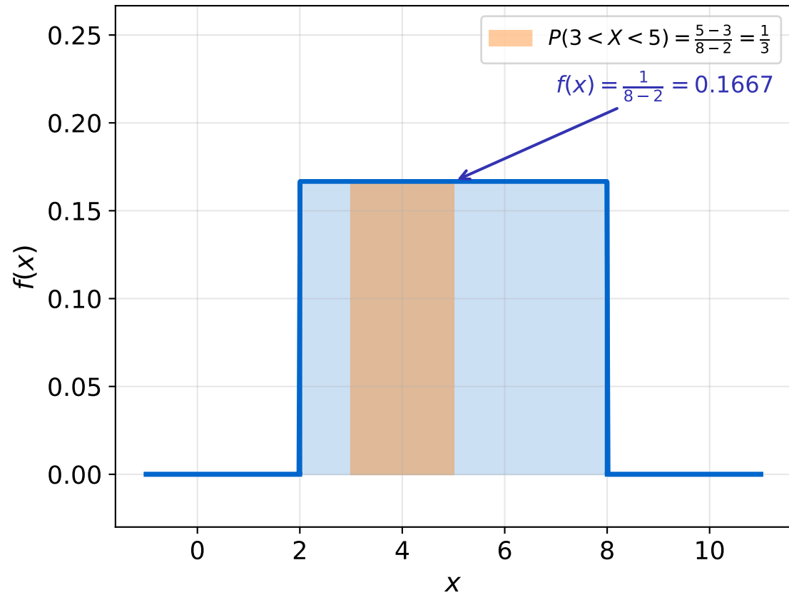
PDF: X \sim U(2, 8)
