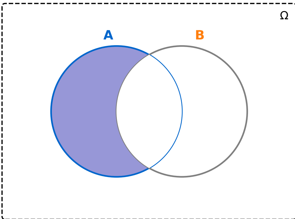
A \setminus B (Differenz)
