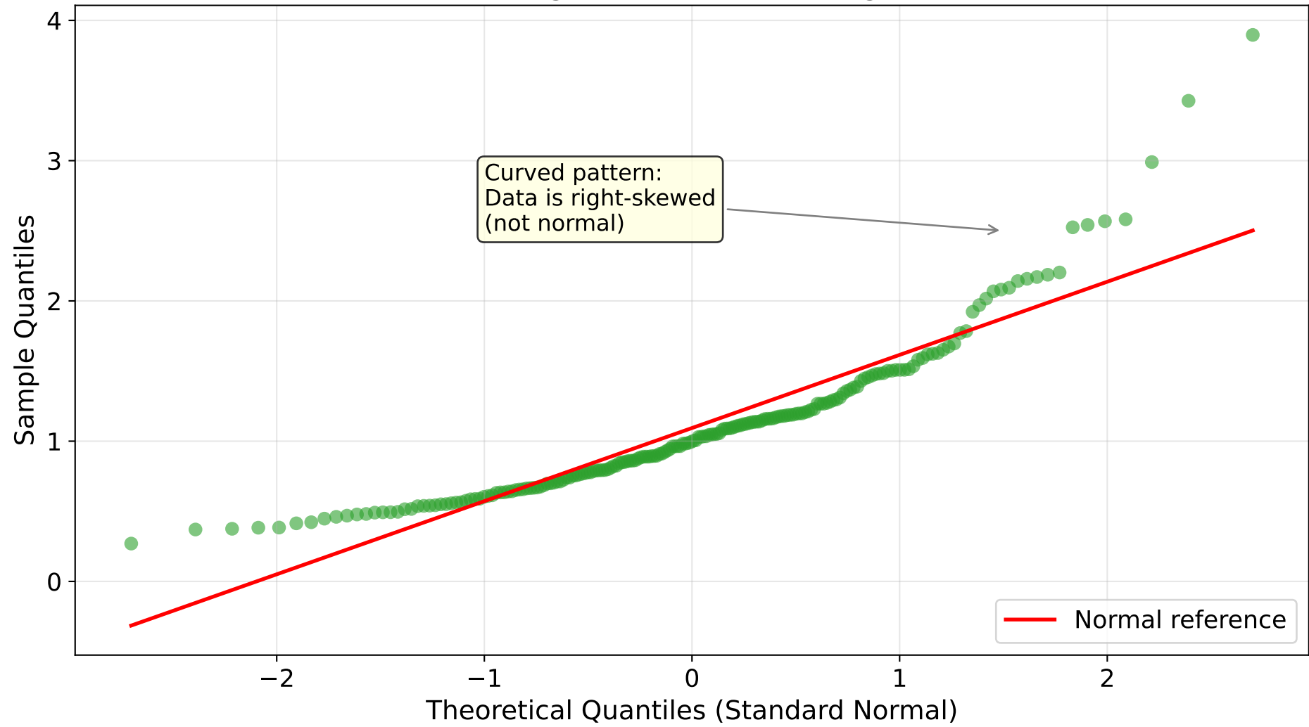
Q-Q Plot: Right-Skewed Data (Log-Normal)
