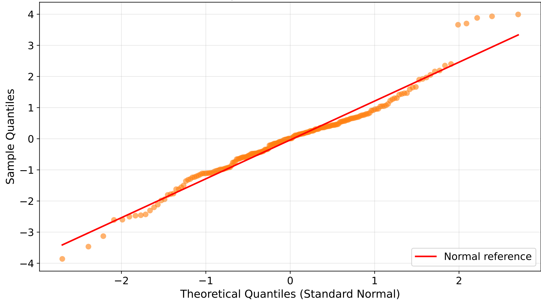
Q-Q Plot: Heavy-Tailed Data (t-distribution, df=3)
