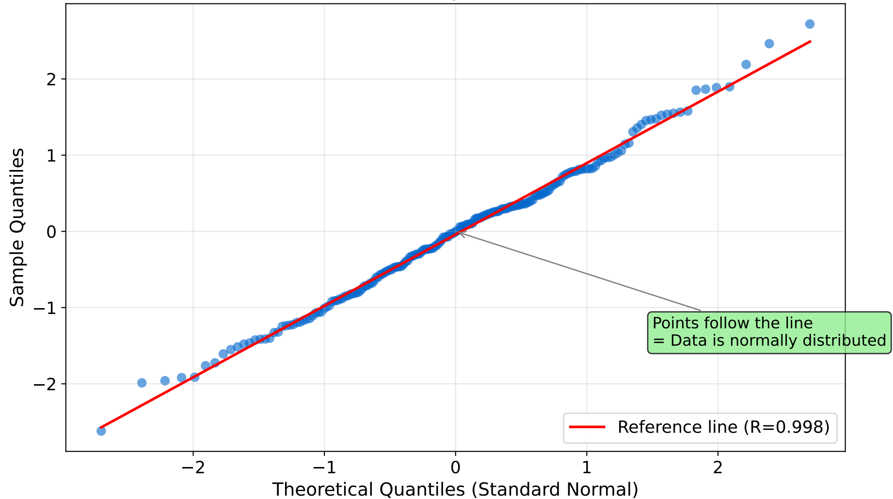
Q-Q Plot: Normally Distributed Data
