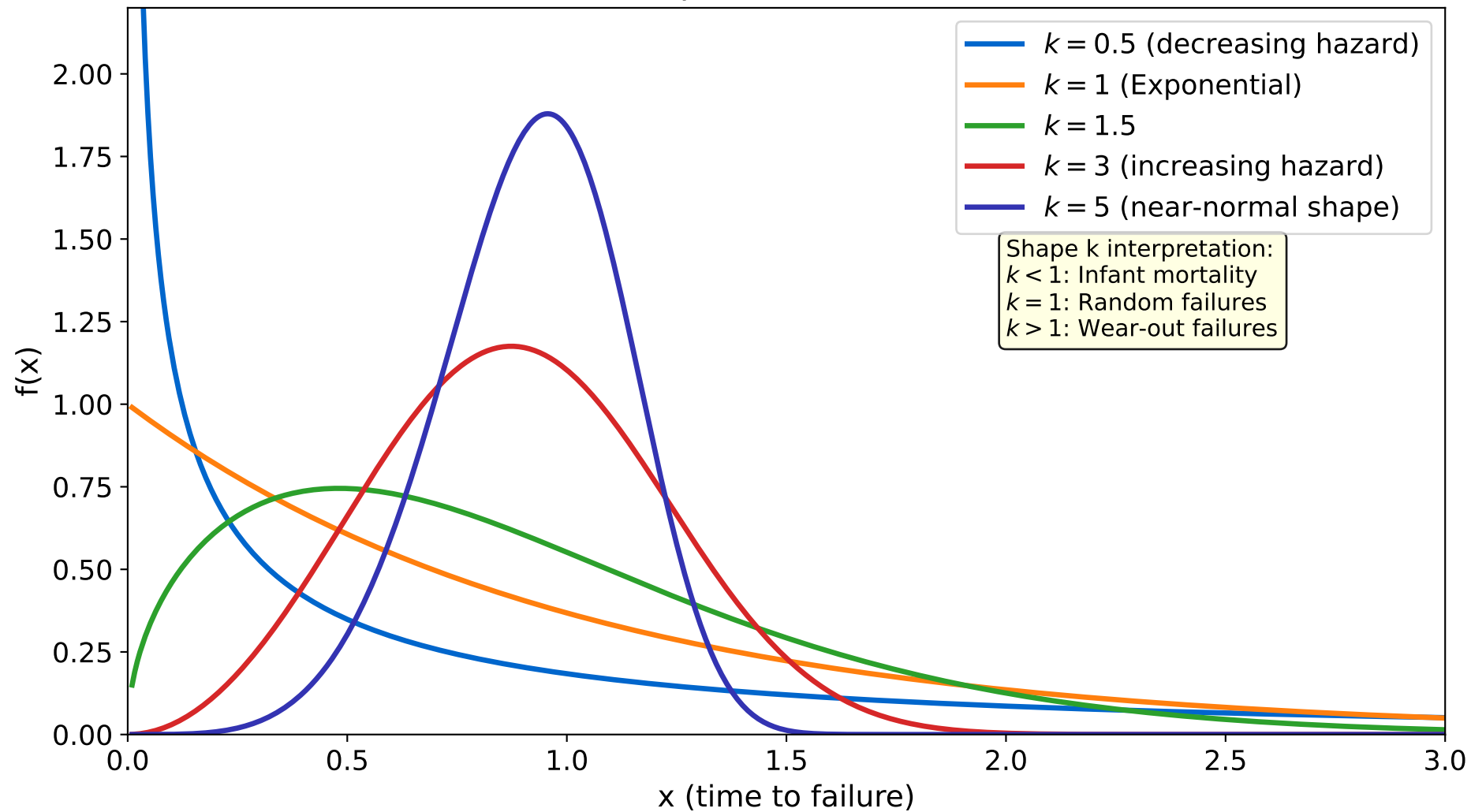
Weibull Distribution: Shape Parameter k Controls Hazard Rate
