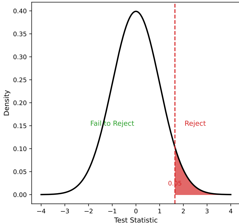
One-Tailed Test (Right) ( \alpha = 0.05 )
