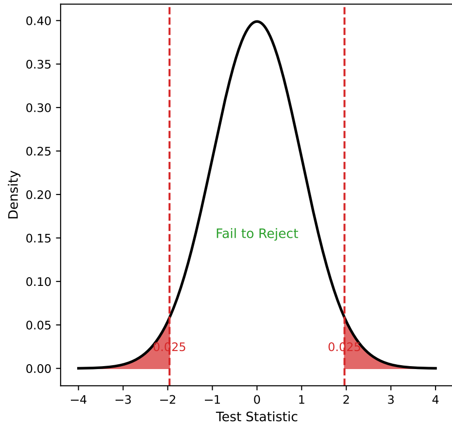
Two-Tailed Test ( \alpha = 0.05 )
