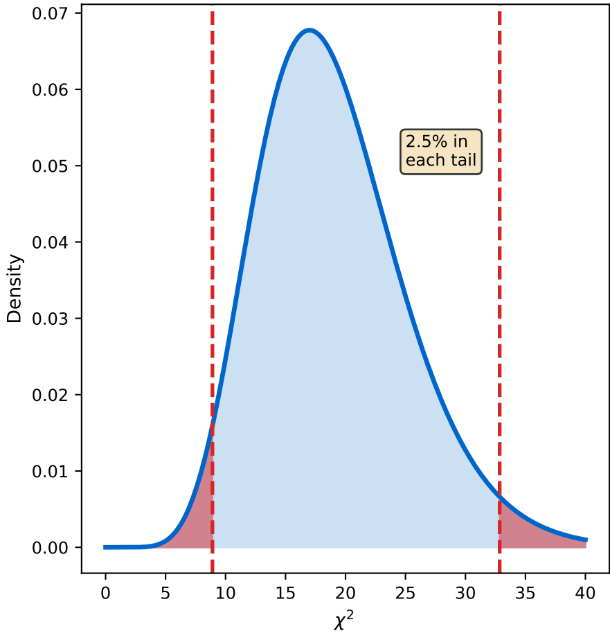
Chi-Square Distribution (df=19)
