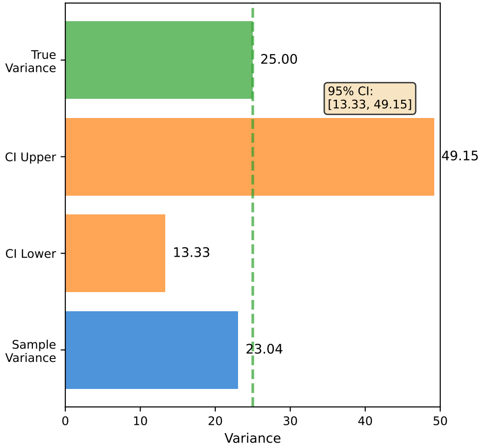
95% CI for Population Variance
