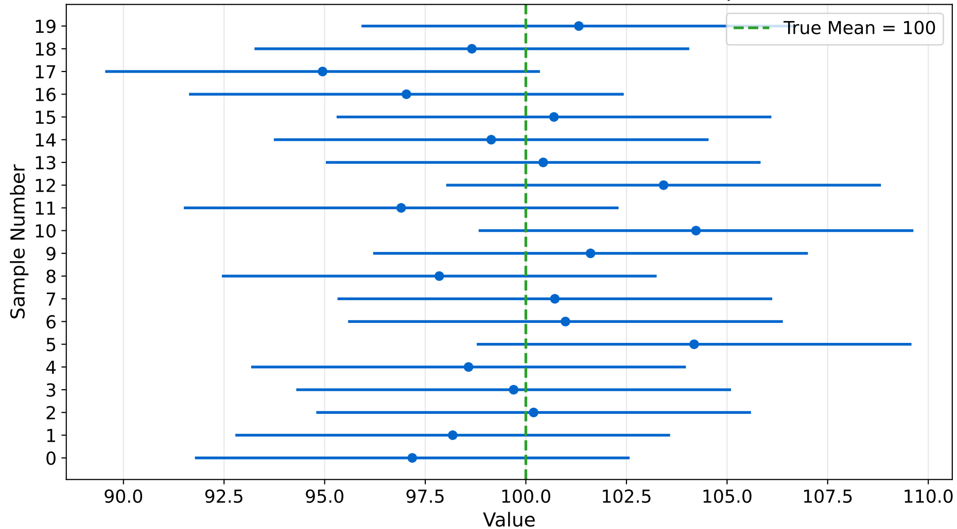
95% Confidence Intervals: 20 Random Samples
