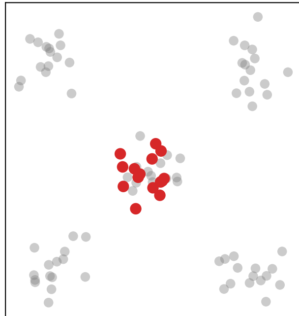
Cluster Sampling
