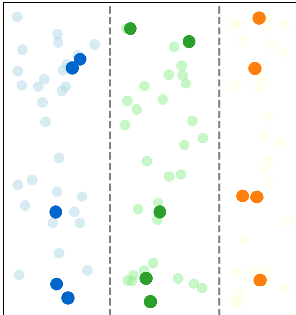
Stratified Sampling
