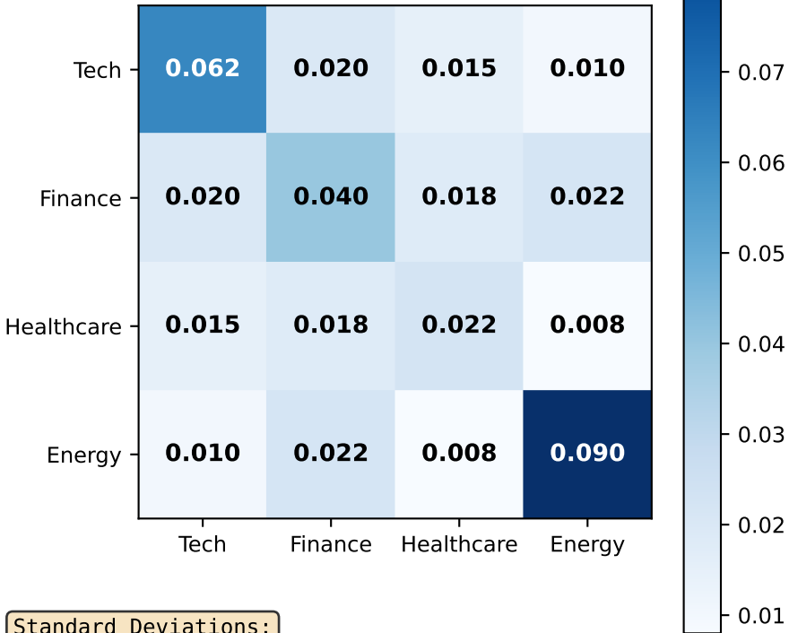
Covariance Matrix
